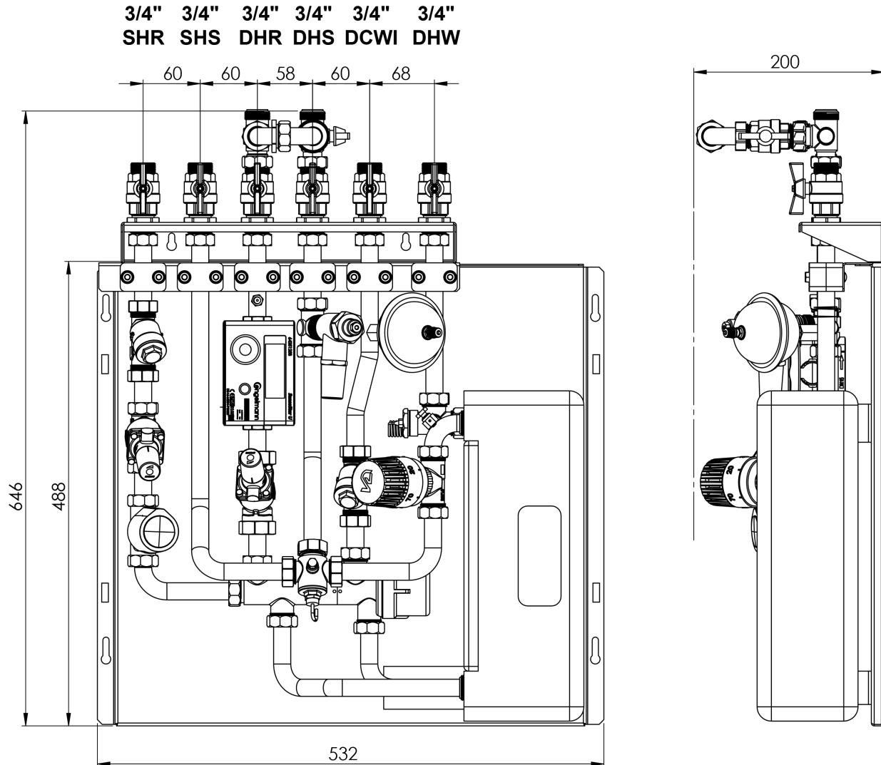
Front View
