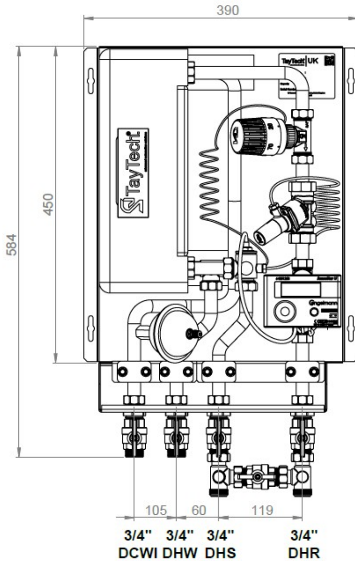
Front View
