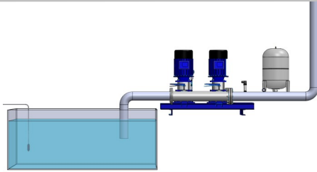
Pressure Transmitter
